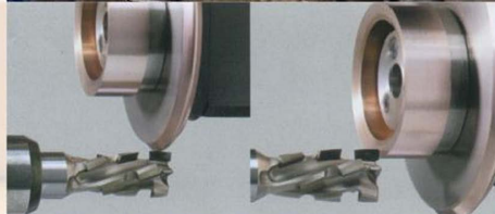
PCD五轴联动数控磨床
